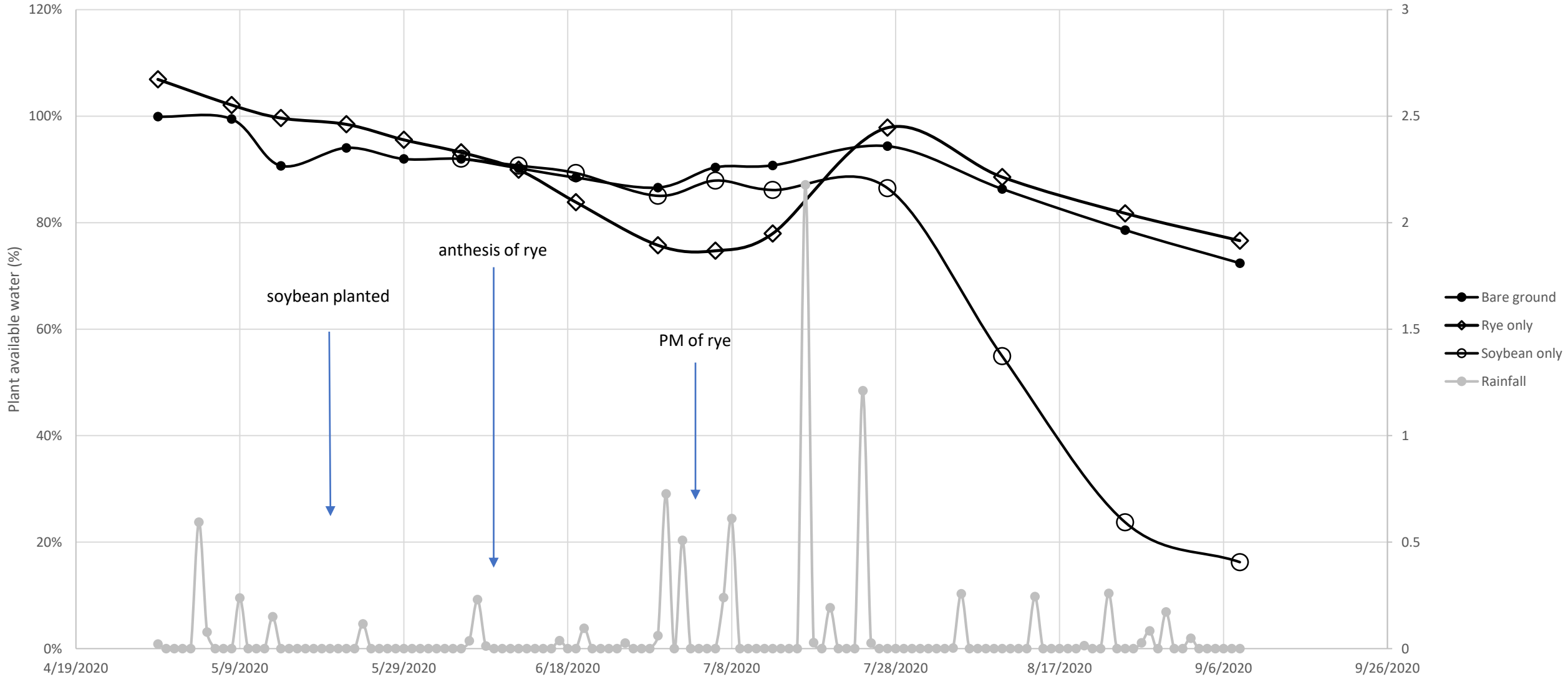
Plant available water status of soil under rye and soybean planted areas or bare ground in 2020
