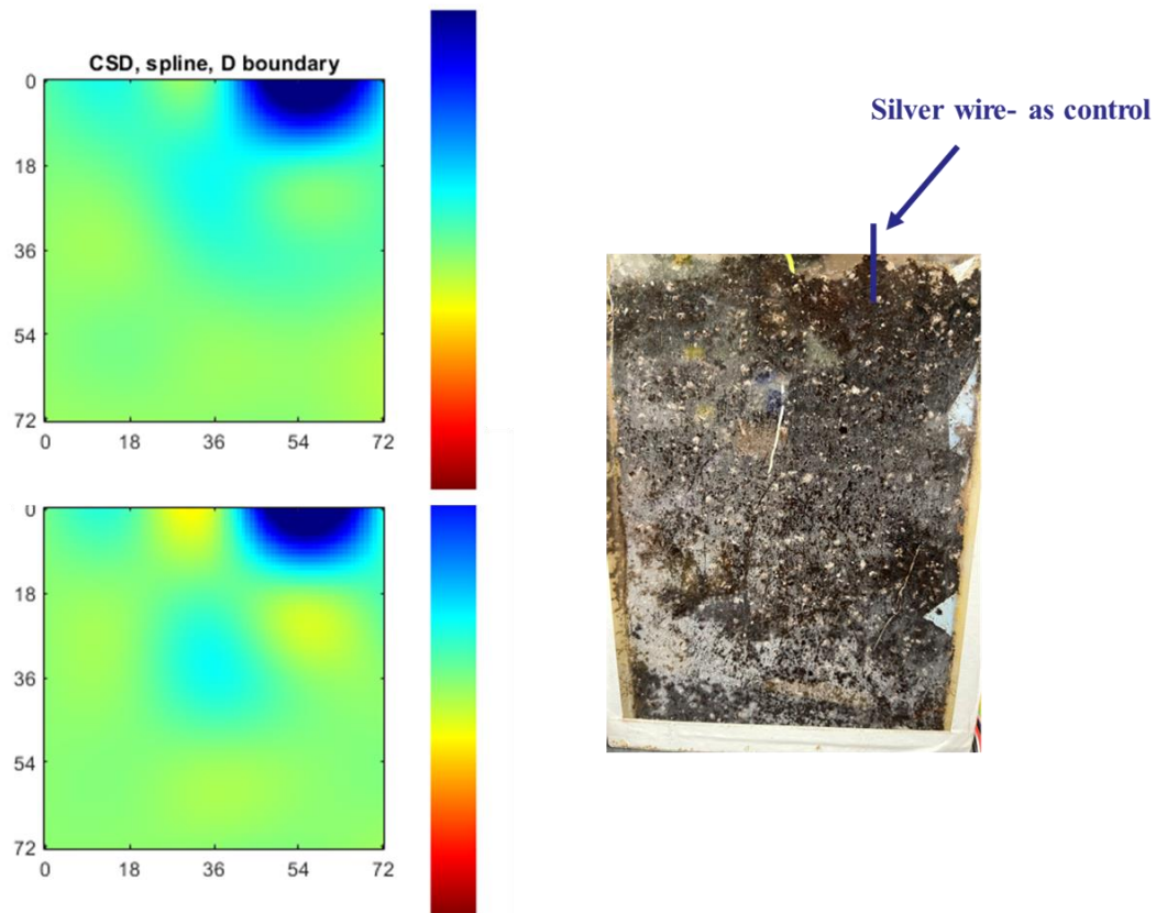
Figure 3: Images of potential induced due to silver wire as control. The images do not have a significant change over 10 days indicating the change observed in the root images is due to the root growth.
