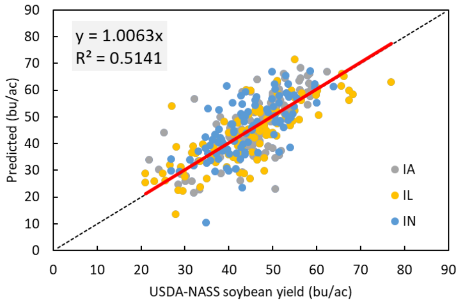
Fig 1 – simulated versus USDA-NASS yield for IA, IL and IN.
