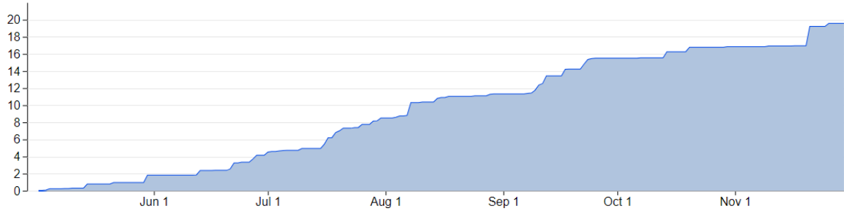
Accumulated Precipitation
