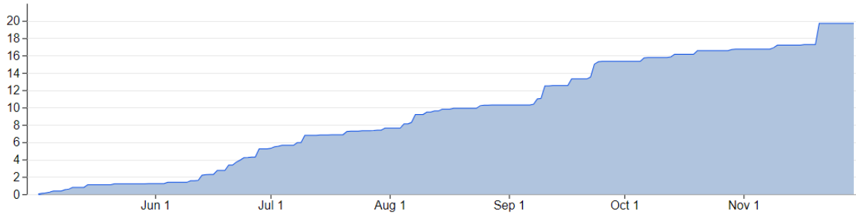
Accumulated Precipitation
