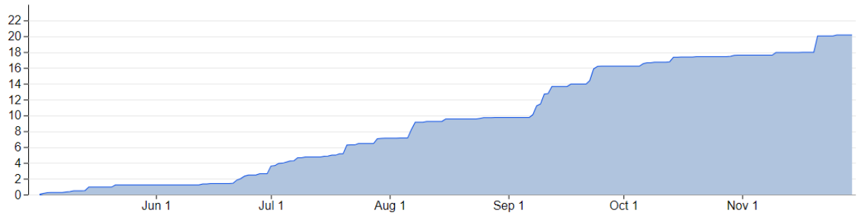
Accumulated Precipitation
