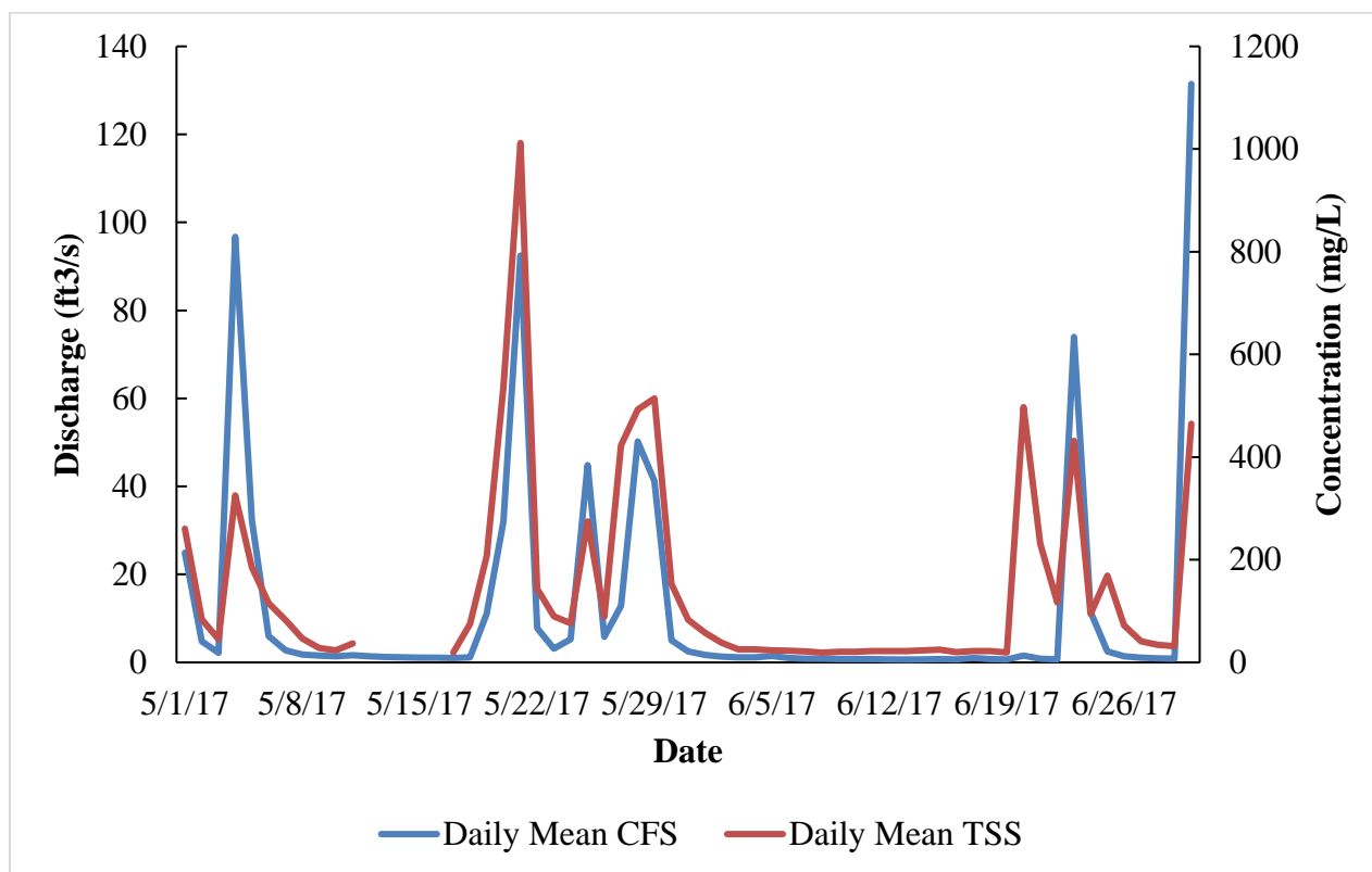
Figure 16. Relationship between stream discharge (primary Y-axis) and total suspended sediment (secondary Y-axis) during the months of May-June 2017. Target value is 30 mg/L.
