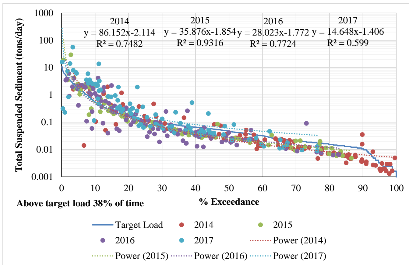
Figure 17. Flow-duration analysis for tons/day of Total Suspended Sediment from 2014-2017 for the Beargrass Creek PWS gage station. The blue line on the graph represents the target load. The target load was exceeded 38% of the time.
