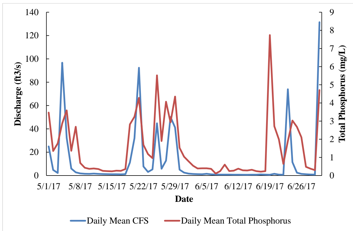
Figure 12. Relationship between stream discharge (primary Y-axis) and Total Phosphorus (secondary Y-axis) during the months of May-June 2017 at the Beargrass Creek PWS gage. Target value is 0.076 mg/L.
