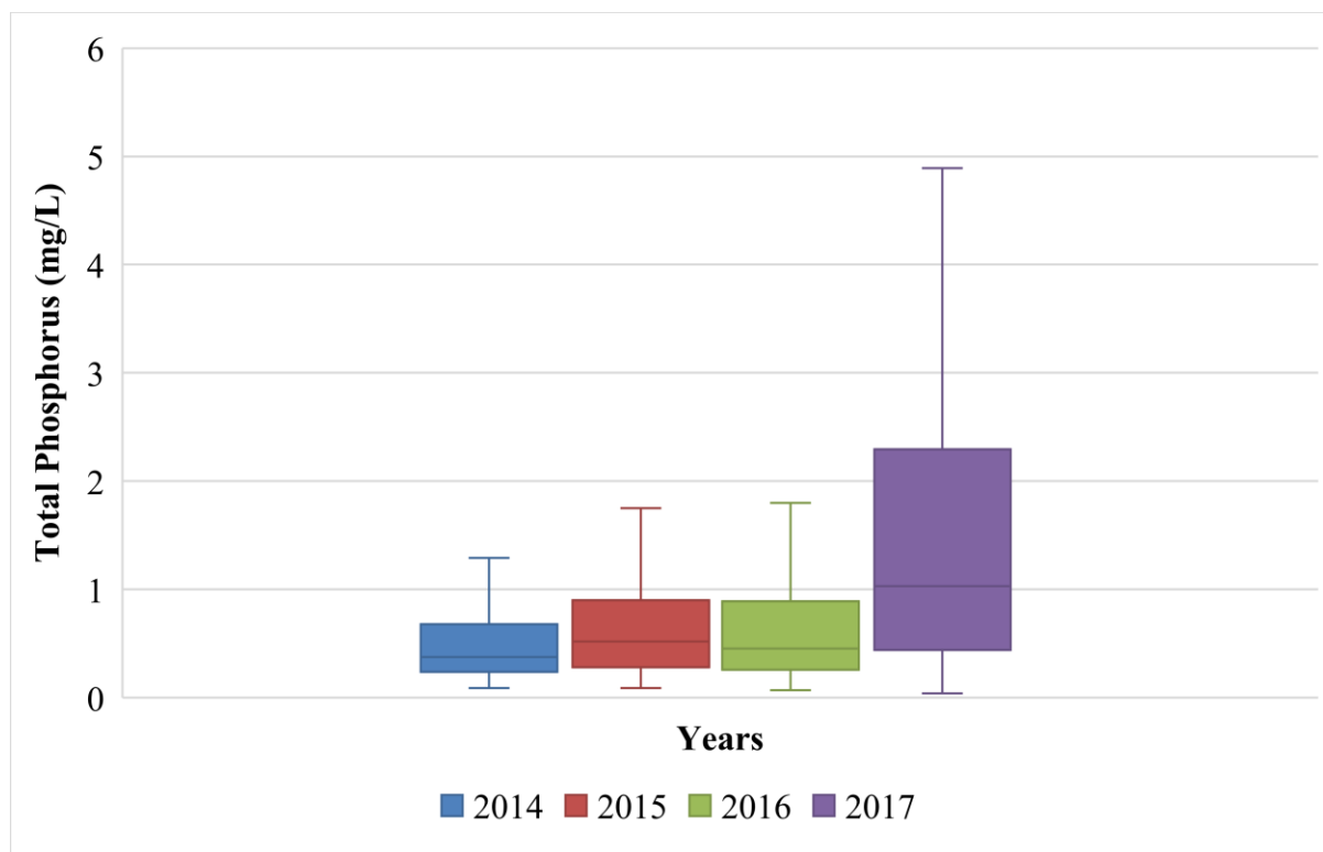
Figure 25. Box and whisker plots for Total Phosphorus at the Pawpaw Creek PWS gage station from 2014-2017. The middle line in the box represents the median value (50 th percentile) for each year. Note the evenness of the medians across the first three years. The target value is 0.076 mg/L.
