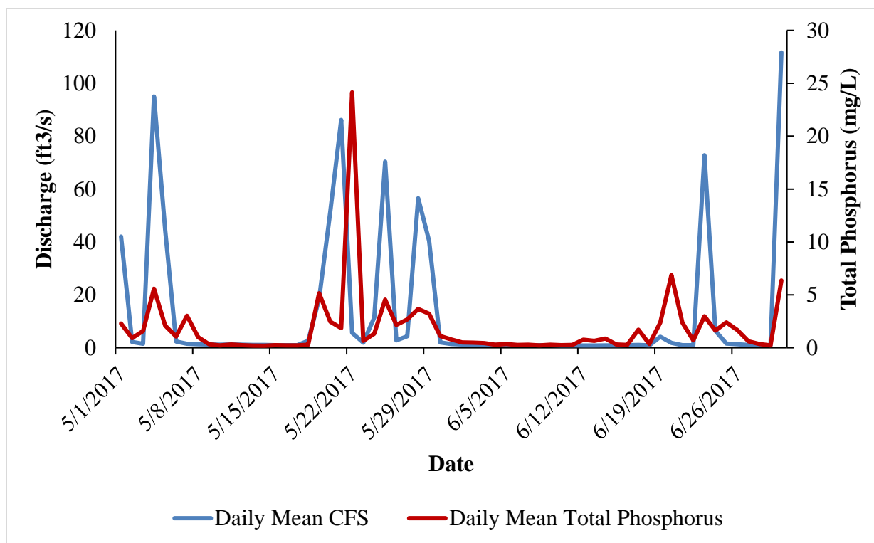
Figure 24. Relationship between stream discharge (primary Y-axis) and Total Phosphorus (secondary Y-axis) during the months of May-June 2017 at the Pawpaw Creek PWS gage. Target value is 0.076 mg/L.
