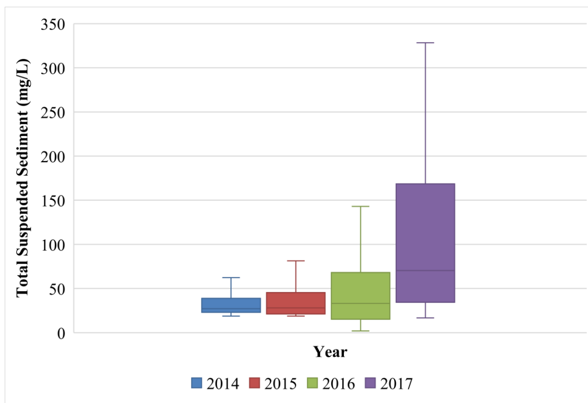
Figure 27. Box and whisker plots for Total Suspended Sediment at the Pawpaw Creek PWS gage station from 2014-2017. The middle line in the box represents the median value (50 th percentile) for each year. Note the upward trend in the median and maximum values. The target value is 30 mg/L.
