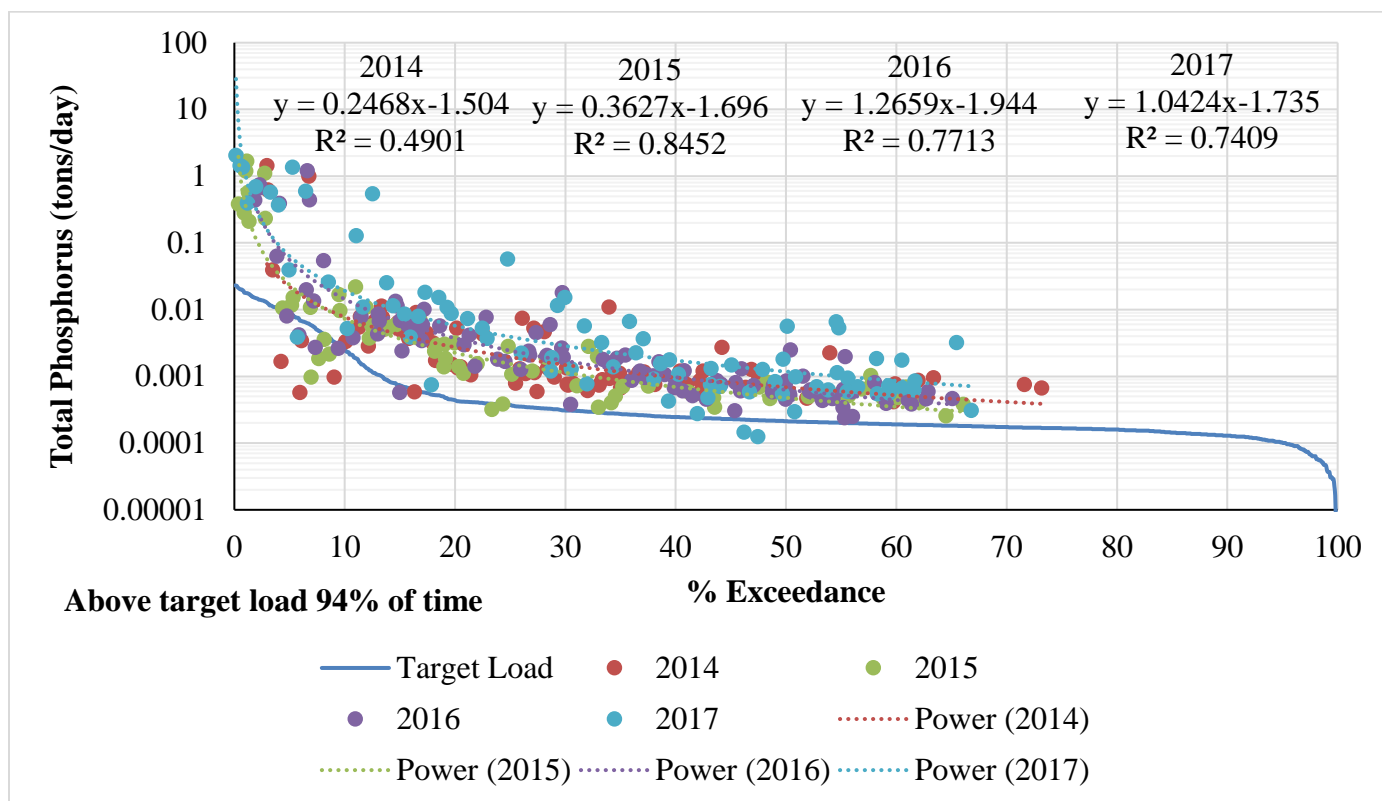
Figure 26. Flow-duration analysis for tons/day of Total Phosphorus from 2014-2017 for the Pawpaw Creek PWS gage station. The blue line on the graph represents the target load. The target load was exceeded 94% of the time.
