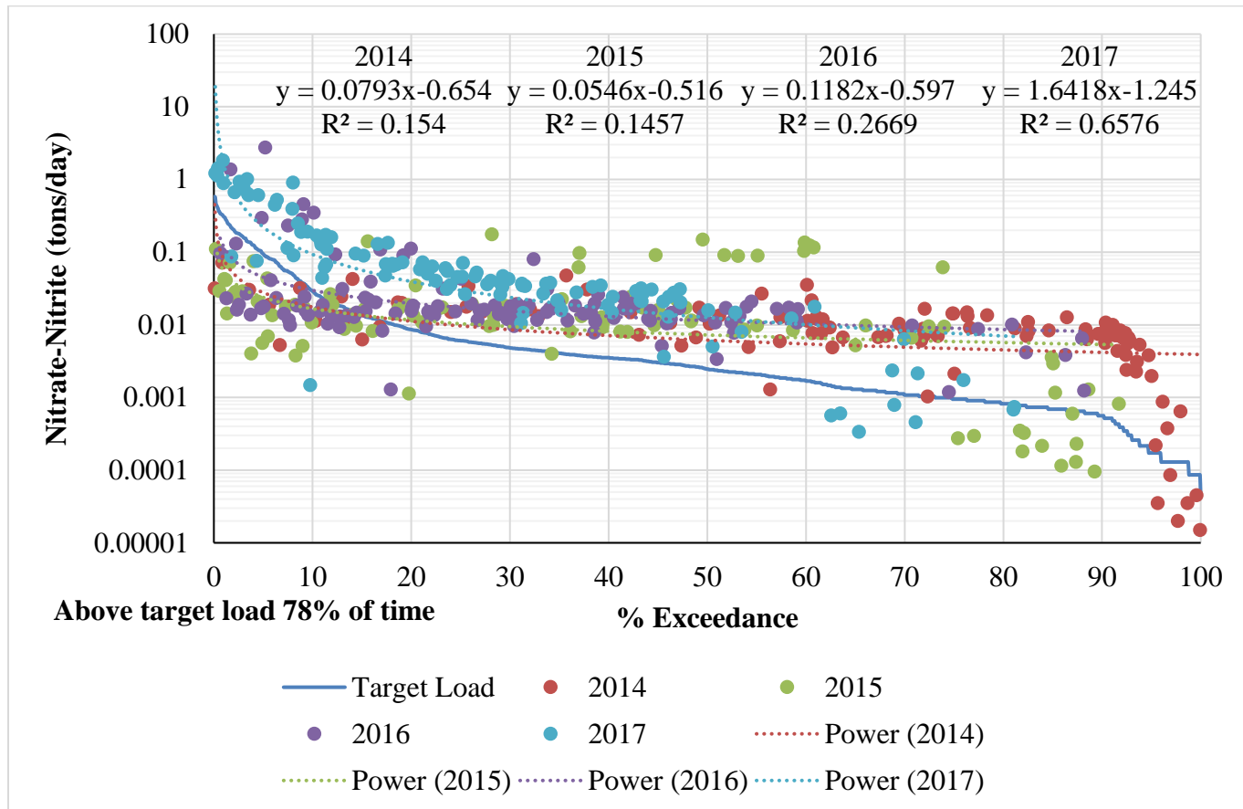
Figure 11. Flow-duration analysis for tons/day of Nitrate-Nitrite from 2014-2017 for Beargrass Creek PWS gage station. The blue line on the graph represents the target load. The target load was exceeded 78% of the time.
