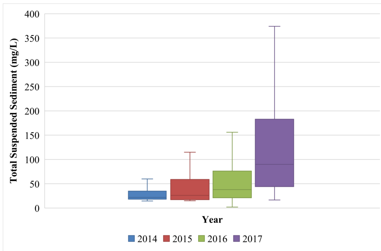
Figure 15. Box and whisker plots for Total Suspended Sediment at the Beargrass PWS gage station from 2014-2017. The middle line in the box represents the median value (50 th percentile) for each year. Note the upward trend in the median and maximum values. The target value is 30 mg/L.
