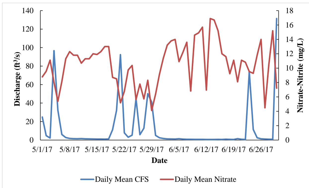
Figure 10. Relationship between stream discharge (primary Y-axis) and nitrate (secondary Y-axis) during the months of May-June 2017 for Beargrass Creek PWS. Target value is 1.6 mg/L.
