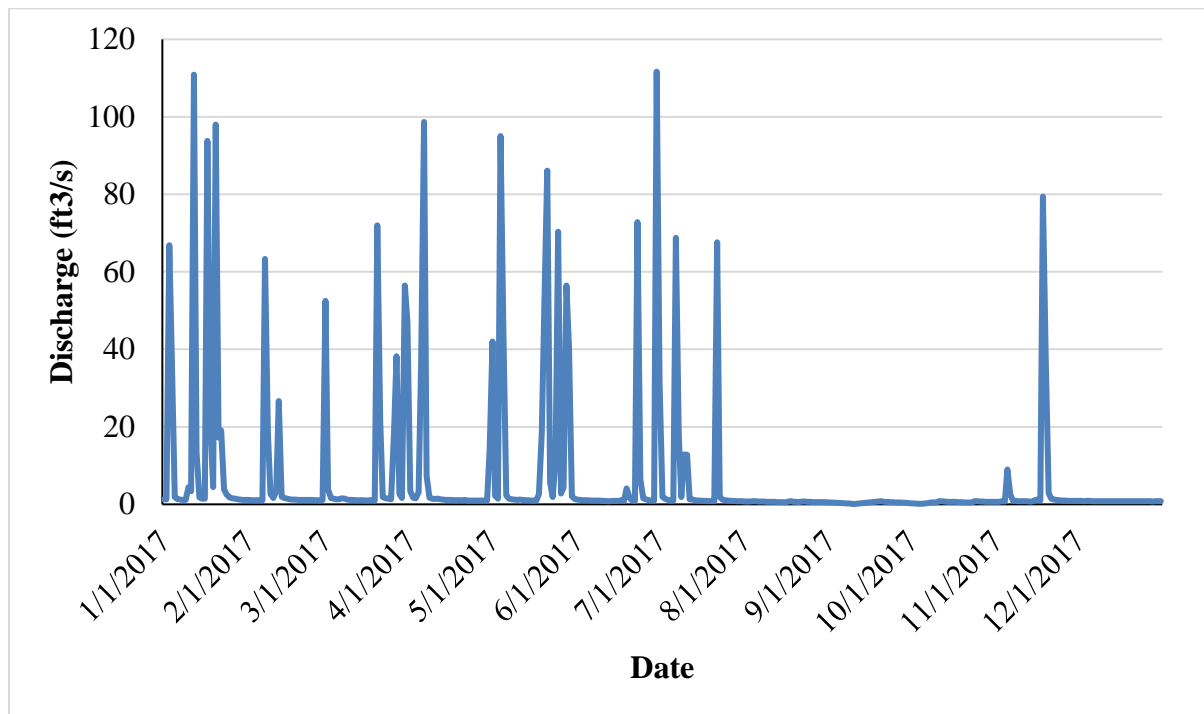
Figure 20. Hydrograph for Pawpaw Creek PWS for 2017. This graph illustrates the temporal variability of stream discharge. May-June was the wettest since keeping records. One cubic foot equals 7.5 gallons.
