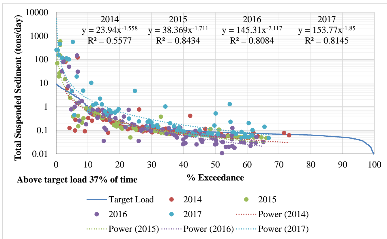
Figure 29. Flow-duration analysis for tons/day of Total Suspended Sediment from 2014-2017 for the Pawpaw Creek PWS gage station. The blue line on the graph represents the target load. The target load was exceeded 37% of the time.
