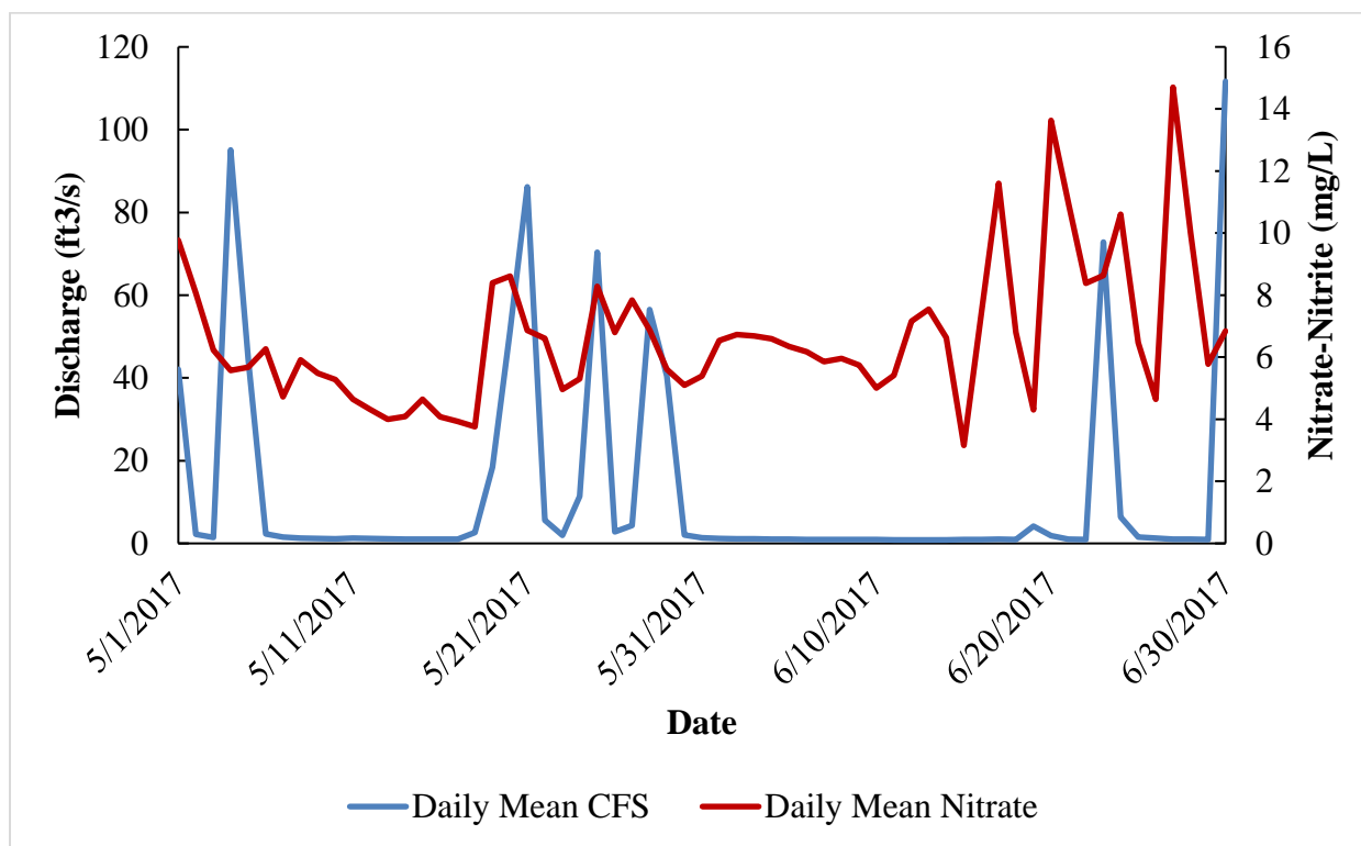
Figure 22. Relationship between stream discharge (primary Y-axis) and nitrate (secondary Y-axis) during the months of May-June 2017 for Pawpaw creek PWS. Target value is 1.6 mg/L.
