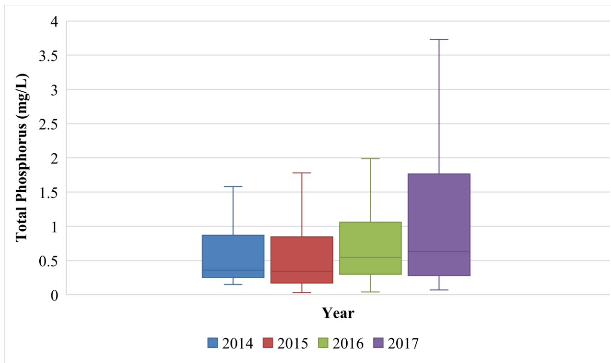
Figure 13. Box and whisker plots for Total Phosphorus at the Beargrass PWS gage station from 2014-2017. The middle line in the box represents the median value (50 th percentile) for each year. Note the evenness of the medians across years. The target value is 0.076 mg/L.
