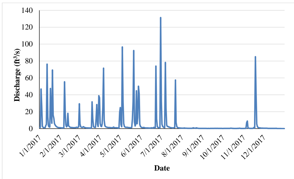
Figure 8. Hydrograph for Beargrass Creek PWS for 2017. This graph illustrates the temporal variability of stream discharge. May-June was the wettest since keeping records. One cubic foot equals 7.5 gallons.
