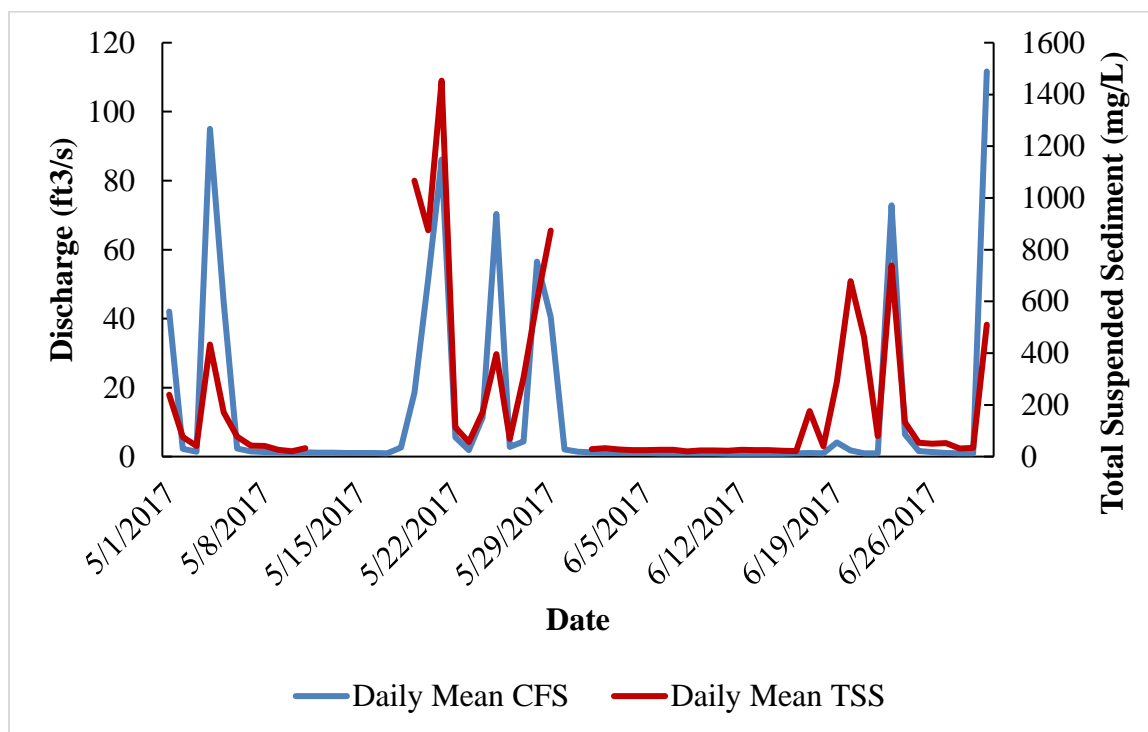
Figure 28. Relationship between stream discharge (primary Y-axis) and total suspended sediment (secondary Y-axis) during the months of May-June 2017 for Pawpaw Creek PWS. Target value is 30 mg/L.
