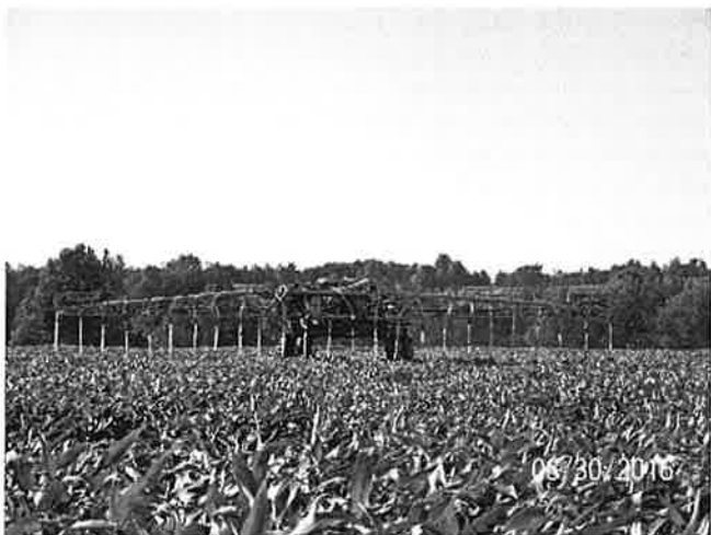
Image 5. Highboy cover crop interseeder.
