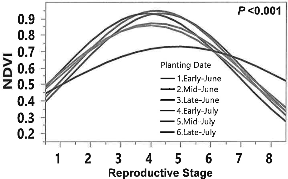
Figure 5. Normalized difference vegetation index (NDVI) over time, as represented by reproductive stage, to planting date of double-crop soybean.
